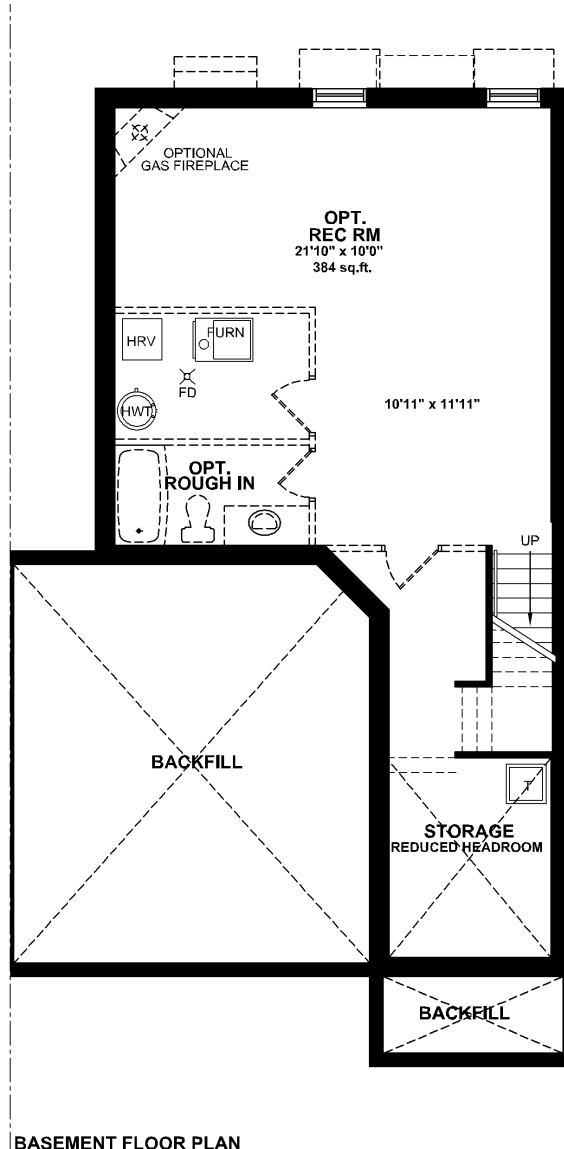
BASEMENT FLOOR PLAN OPTIONAL FINISHED BASEMENT = 384 SQ.FT. (+55 SQ.FT. BATHRM)
