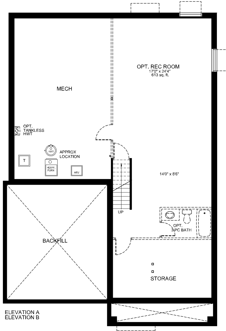
BASEMENT FLOOR PLAN OPTIONAL FINISHED BASEMENT = 613 SQ.FT. (+48 SQ.FT. BATHRM)
