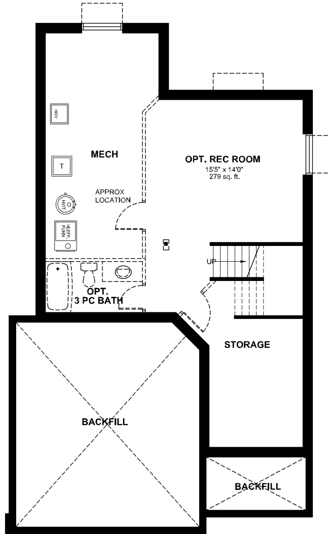
BASEMENT FLOOR PLAN 279 SQ. FT. FINISHED AREA-OPTIONAL
