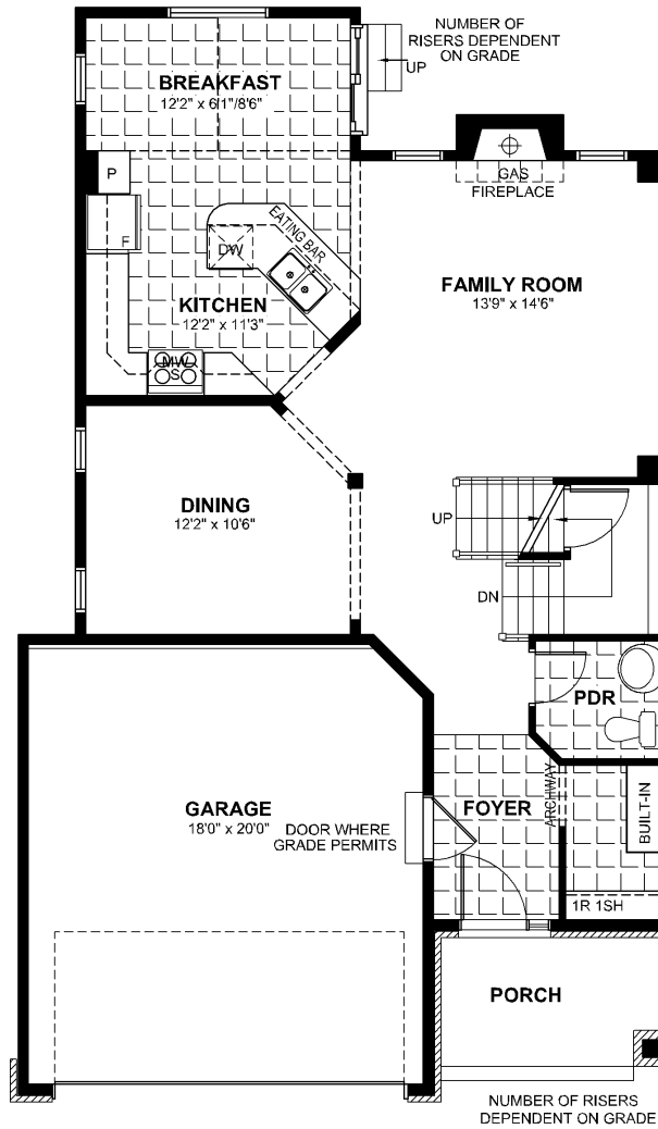
ELEVATION 'A' & 'B' GROUND FLOOR PLAN 853 SQ. FT.
