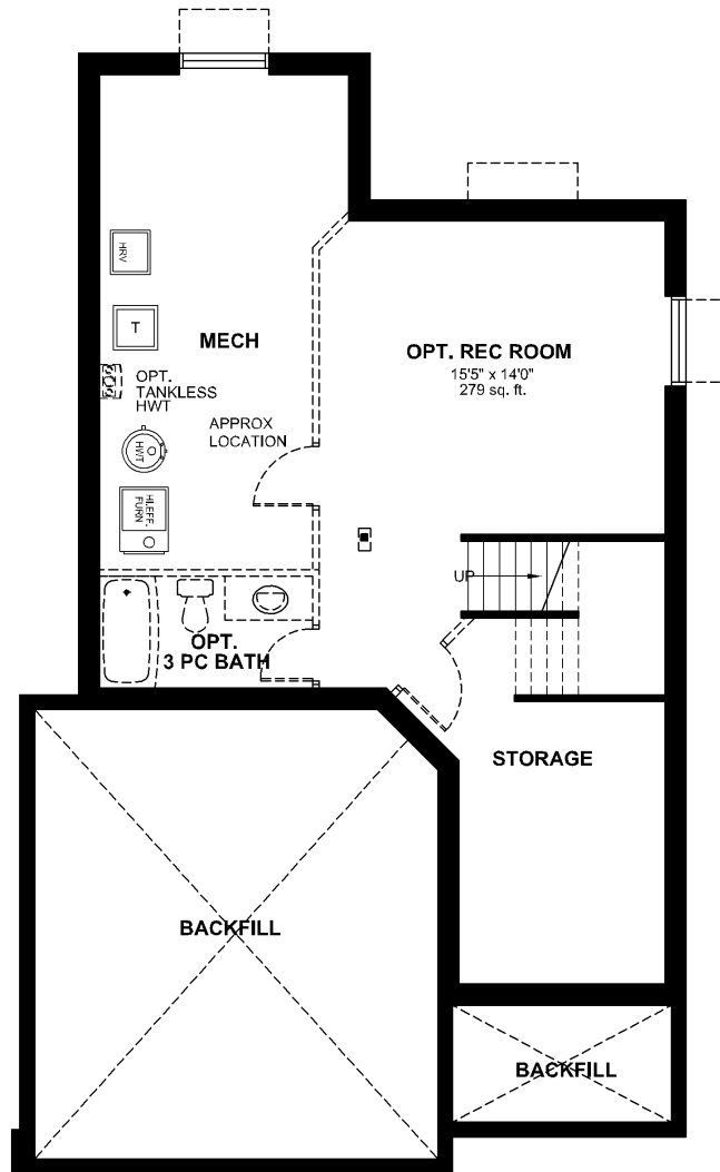
BASEMENT FLOOR PLAN OPTIONAL FINISHED BASEMENT = 279 SQ.FT. (+52 SQ.FT. BATHRM)
