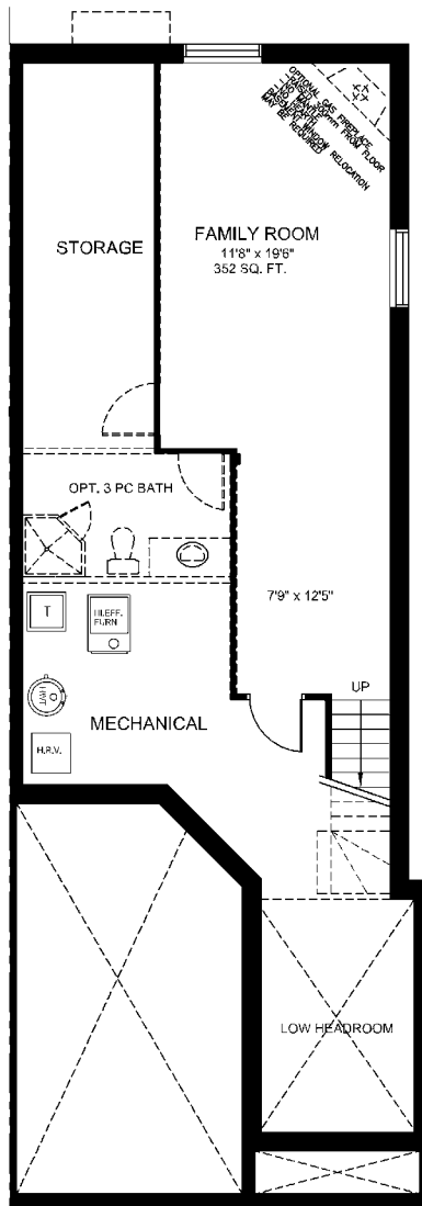
BASEMENT FLOOR PLAN FIN. AREA= 352 SQ. FT.
