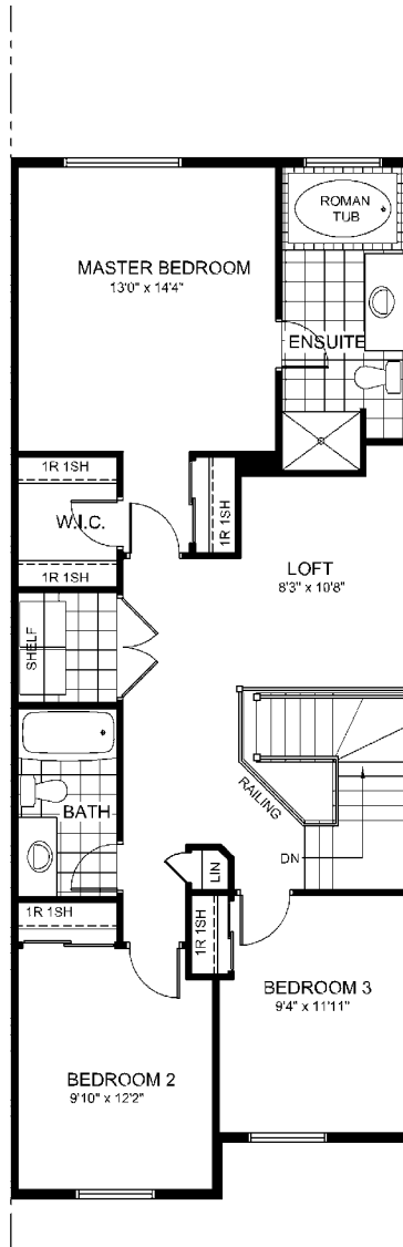
SECOND FLOOR PLAN 1034-14 = 1020 SQ. FT.
