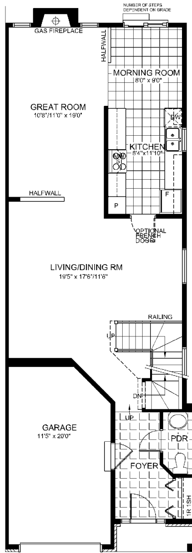
GROUND FLOOR PLAN 954 SQ. FT.
